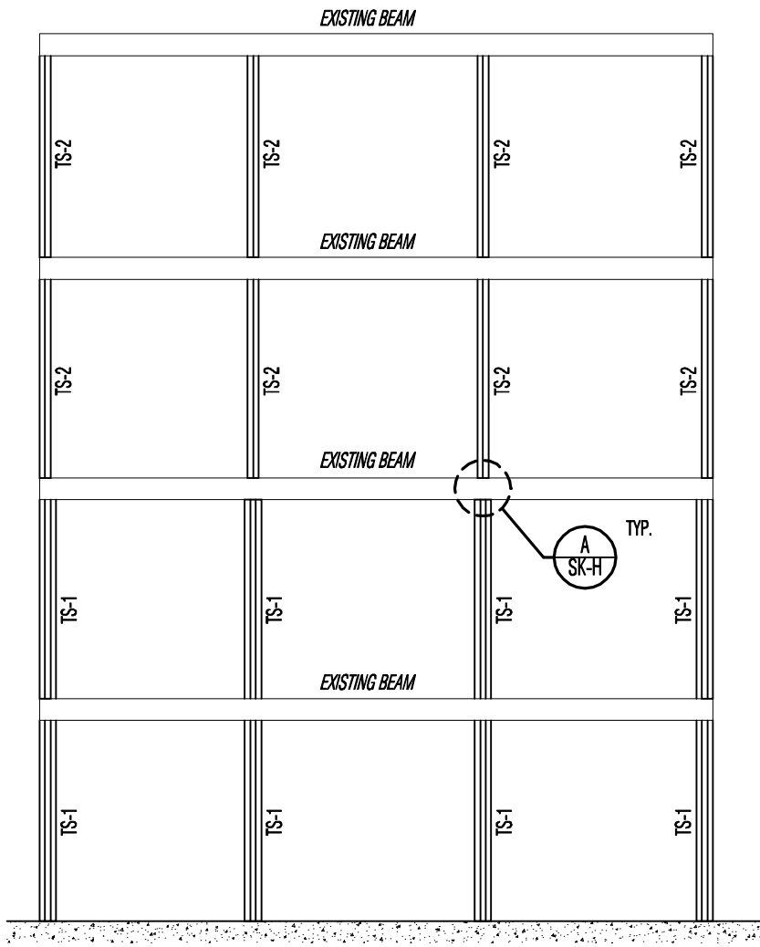
2 FRONT ELEVATION OF BALCONIES
